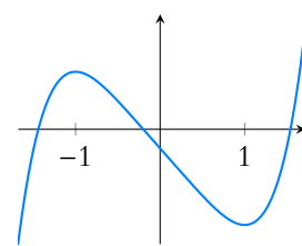
FIGURE 7.1– x \mapsto x^5 - 5x - 1 .
